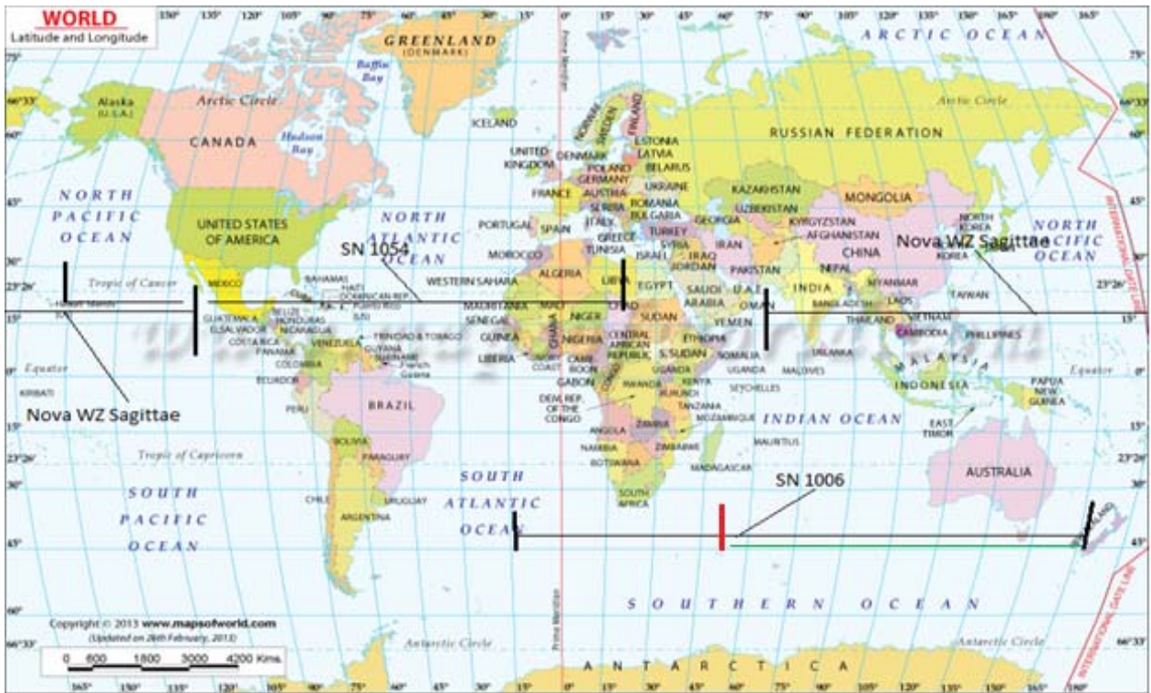
Fig. 11 Heating paths and termini—Nova WZ Sagittae, SN 1006, SN 1054 [29].
