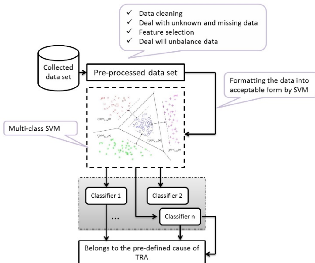
Fig. 1 The framework of predicting the cause of road traffic accident using multi-class SVMs.
